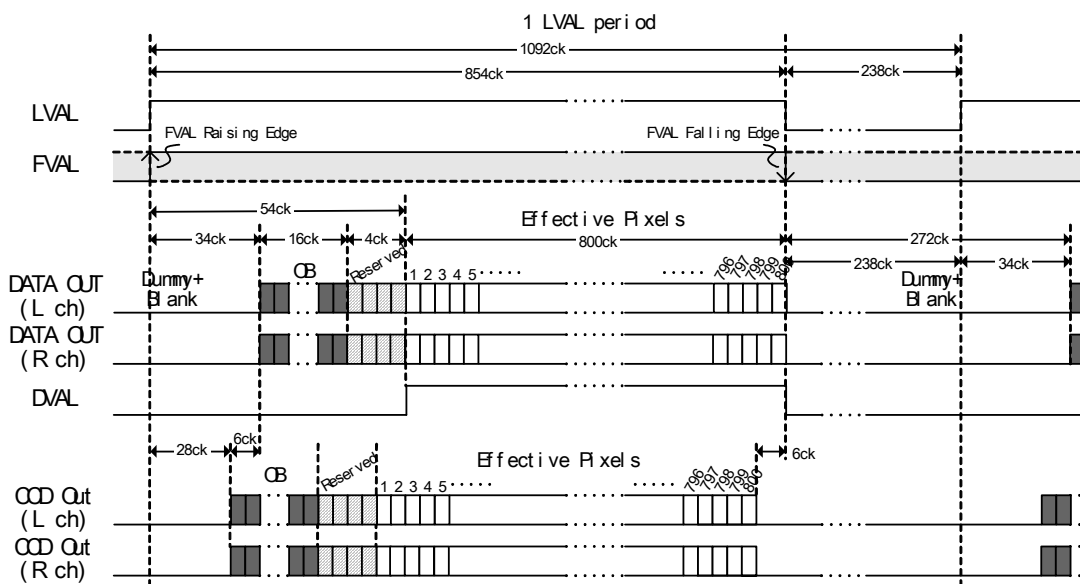
Fig. 20. Horizontal timing details dual channel
